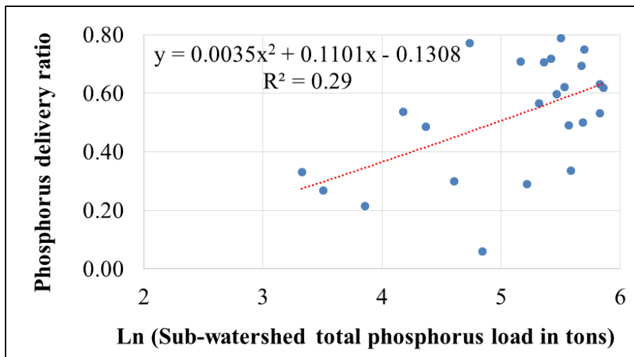
Figure S2 Relationship between sub-watershed pollutant load and delivery ratios (a) Sediment (b) Total nitrogen and (c) Total phosphorus
