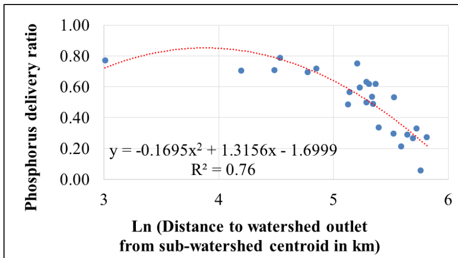
Figure S3 Relationship between sub-watershed distance to watershed outlet and delivery ratios (a) Sediment (b) Total nitrogen and (c) Total phosphorus
