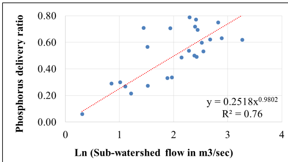
Figure S1 Relationship between sub-watershed flow and delivery ratios (a) Sediment (b) Total nitrogen and (c) Total phosphorus
